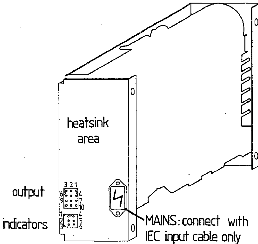
8A power supply unit : low voltage connectors
